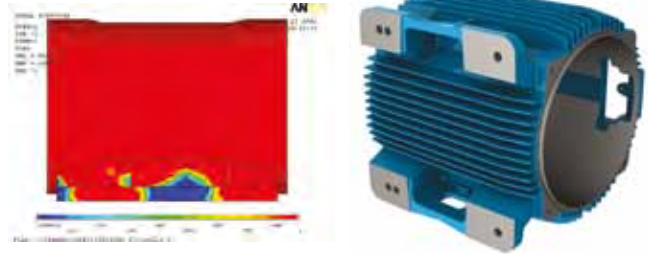
Figure 2 – Solid feet
